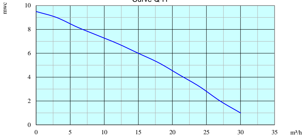
Curve Q-H
